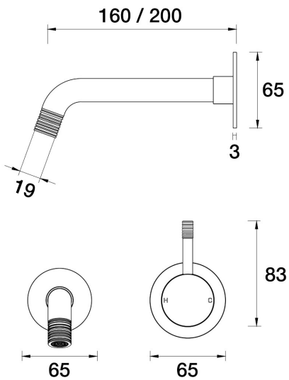
Elm Lane Wall Mixer Basin Set 200mm outlet A42.032.4.57 - Matt Nickel
