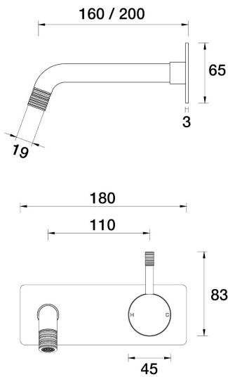
Elm Lane Wall Bath Mixer Set 160mm outlet Incl. plate A42.041.1.52 - Burnished
