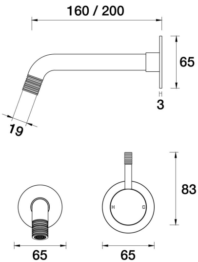
Elm Lane Wall Bath Mixer Set 160mm No Back Plate Part No. 41.2.01 - Chrome
