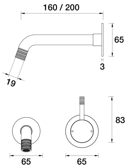
Elm Lane Wall Bath Mixer Set 160mm outlet A42.041.2.57 - Matt Nickel
