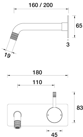
Elm Lane Wall Bath Mixer Set 200mm outlet Incl. plate A42.041.3.19 - 23k Brushed Brass Gold
