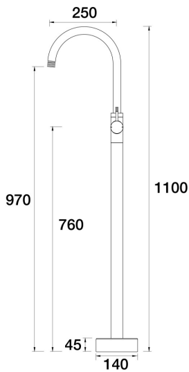
Elm Lane Floor Bath Filler Mixer - Gooseneck A42.072.1.45 - Native Brass
