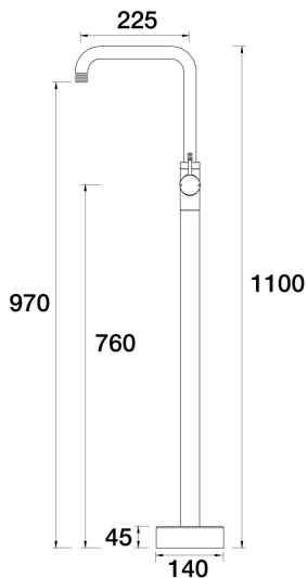
Elm Lane Floor Bath Filler Mixer - 90 Degree A42.073.1.44 - Antique Copper
