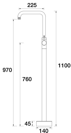
Elm Lane Floor Bath Filler Mixer - 90 Degree A42.073.1.45 - Native Brass
