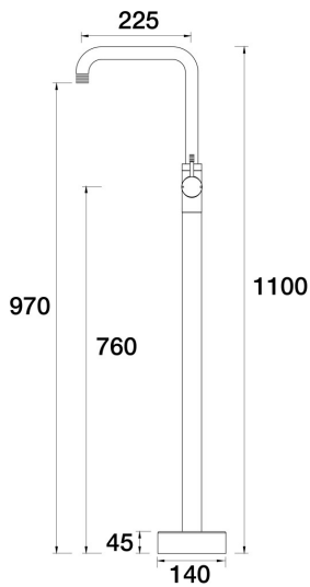
Elm Lane Floor Bath Filler Mixer - 90 Degree A42.073.1.48 - Copper
