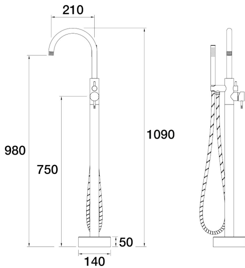
Elm Lane Floor Bath Filler Mixer with Handshower Gooseneck A42.075.1.40 - Rumbled Brass
