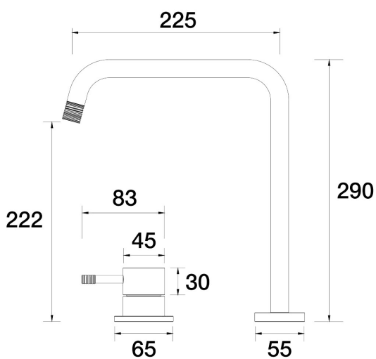
Elm Lane Hob Mixer Set A42.081.2.12 - 23k Brushed Gold
