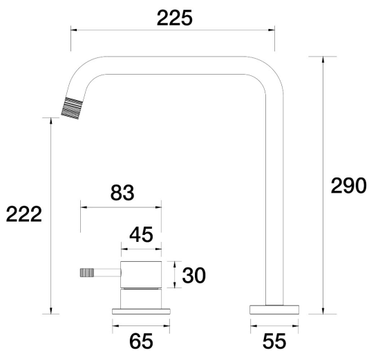
Elm Lane Hob Mixer Set A42.081.2.23 - Gunmetal
