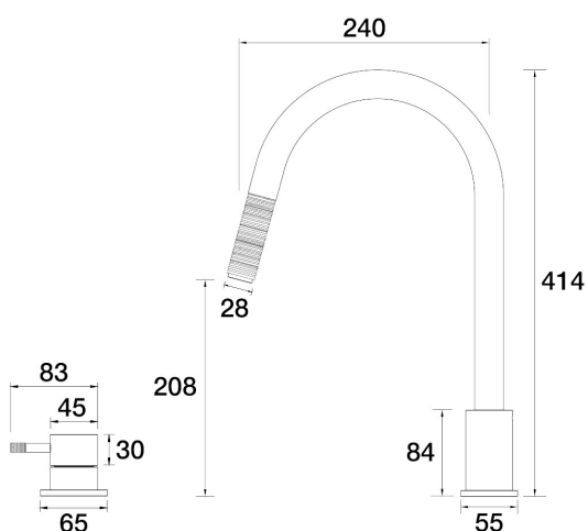
Elm Lane Hob Mixer Pullout Gooseneck Set A42.081.3.23 - Gunmetal
