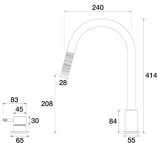
Elm Lane Hob Mixer Pullout Gooseneck Set A42.081.3.25 - Brushed Nickel
