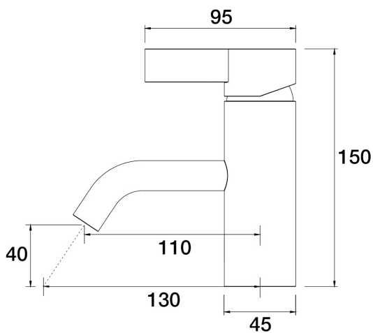
ARI Hob Basin Mini A43.013.1.45 - Native Brass
