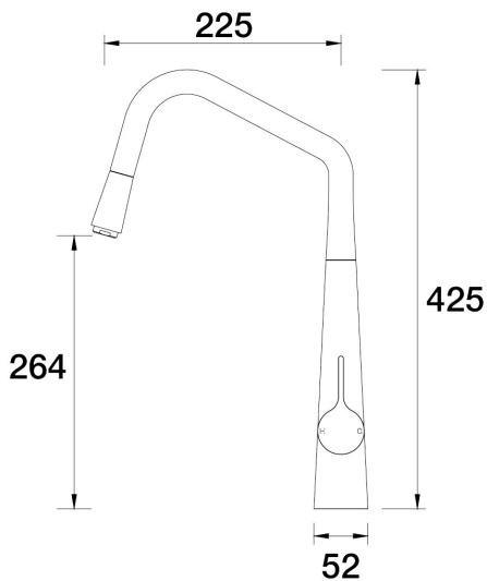
ARI Sink Pull-Out Mixer Upswept A43.024.2.24 - Brushed Gunmetal
