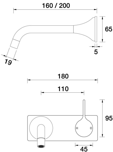
ARI Wall Mixer Basin Set 200mm outlet Incl. plate A43.032.1.01 - Chrome
