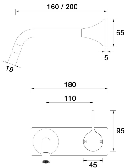
ARI Wall Mixer Basin Set 200mm outlet Incl. plate A43.032.1.27 - Satin Pearl
