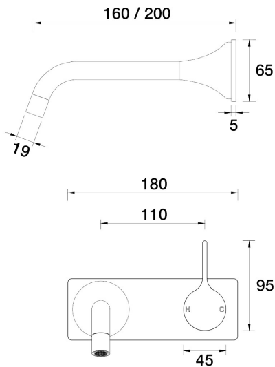
ARI Wall Mixer Basin Set 200mm outlet Incl. plate A43.032.1.54 - Volcanic Grey
