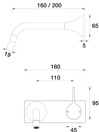
ARI Wall Mixer Basin Set 160mm outlet Incl. plate A43.032.2.25 - Brushed Nickel
