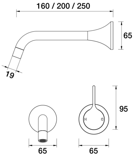
ARI Wall Mixer Basin No Back Plate A43.033.1.01 - Chrome
