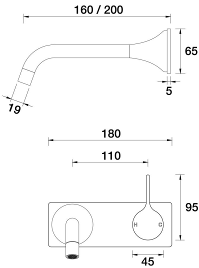
ARI Wall Bath Mixer Set 200mm outlet Incl. plate A43.041.1.01 - Chrome
