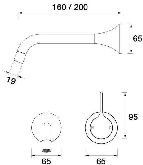
ARI Wall Bath Mixer Set 160mm outlet A43.043.1.43 - Brass
