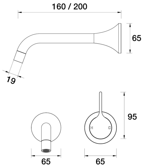
ARI Wall Bath Mixer Set 160mm outlet A43.043.1.52 - Burnished
