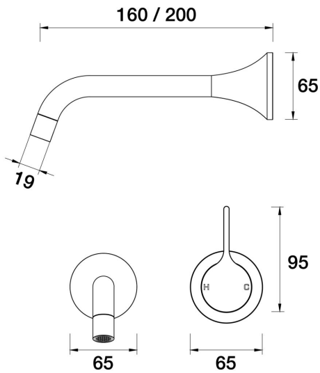
ARI Wall Bath Mixer Set 200mm outlet A43.043.2.01 - Chrome
