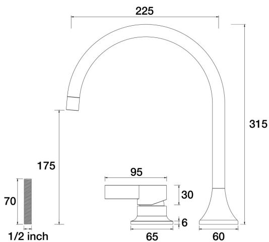
ARI Hob Mixer with Gooseneck Outlet A43.081.2.48 - Copper
