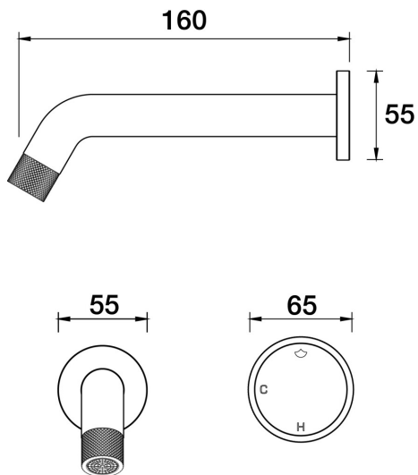
Opus Wall Bath Mixer 160mm A45.041.1.19 - 23k Brushed Brass Gold
