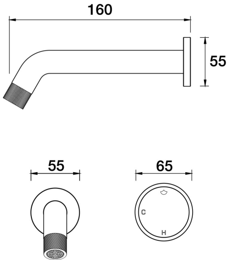
Opus Wall Bath Mixer 160mm A45.041.1.44 - Antique Copper
