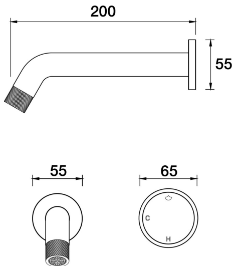
Opus Wall Bath Mixer 200mm A45.042.1.11 - 23k Gold
