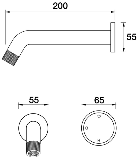
Opus Wall Bath Mixer 200mm A45.042.1.23 - Gunmetal
