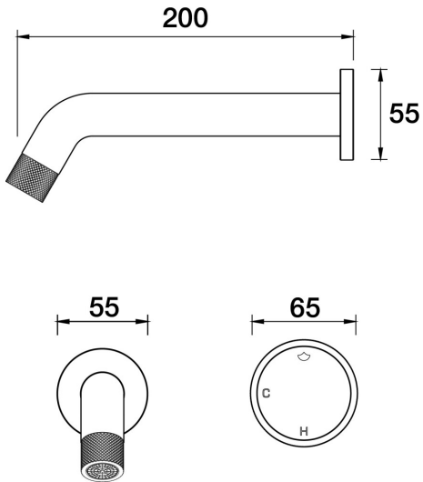
Opus Wall Bath Mixer 200mm A45.042.1.34 - Matt Black
