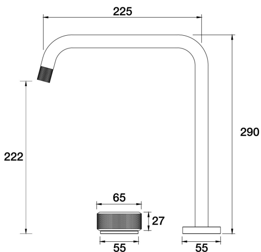
Opus Hob Mixer with Hob Outlet A45.082.1.43 - Brass
