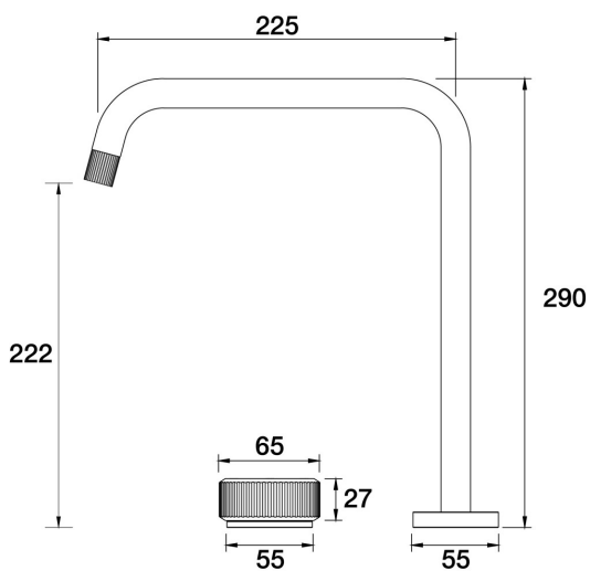
Opus Hob Mixer with Hob Outlet Lane A45.082.2.41 - Brushed Brass
