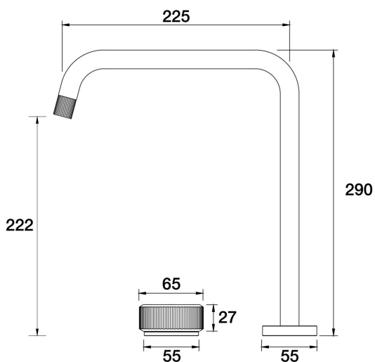
Opus Hob Mixer with Hob Outlet Lane A45.082.2.45 - Native Brass
