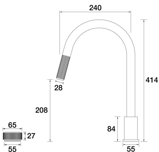
Opus Hob Mixer with Gooseneck Pullout Outlet A45.083.1.01 - Chrome
