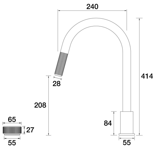
Opus Hob Mixer with Gooseneck Pullout Outlet A45.083.1.24 - Brushed Gunmetal
