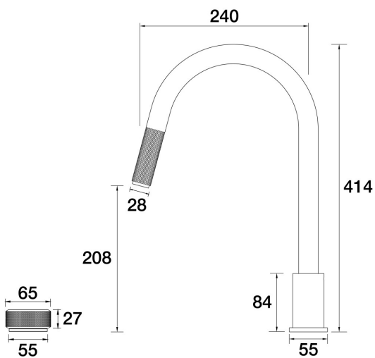
Opus Hob Mixer with Gooseneck Pullout Outlet A45.083.1.32 - Midnight Black
