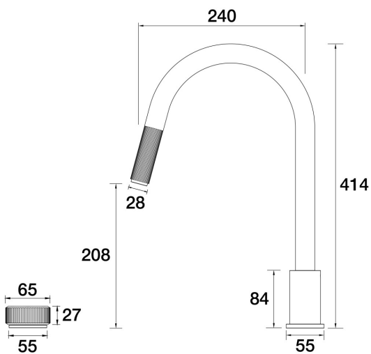
Opus Hob Mixer with Gooseneck Pullout Outlet Part No. 83.2.32 - Midnight Black
