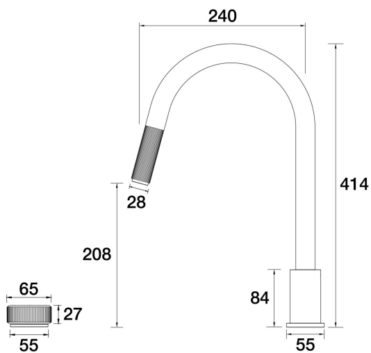
Opus Hob Mixer with Gooseneck Pullout Outlet Part No. 83.2.44 - Antique Copper
