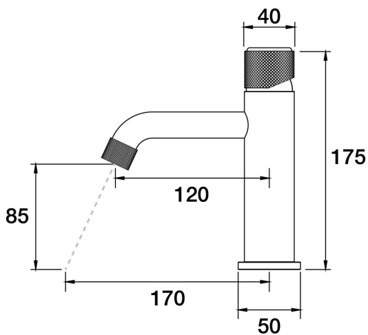
IDK Vetro Hob Basin Mixer A48.011.1.41 - Brushed Brass
