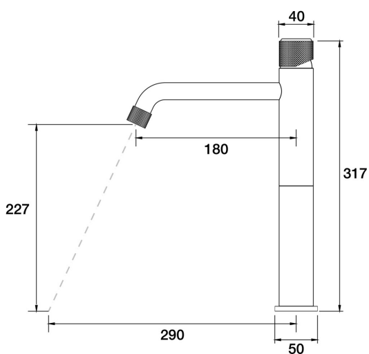
IDK Vetro Hob Basin Tower Mixer A48.012.1.57 - Matt Nickel
