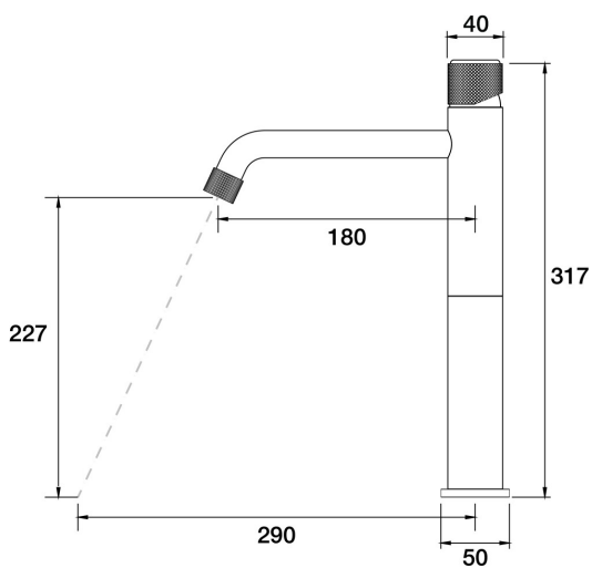
IDK Vetro Hob Basin Tower Mixer A48.012.1.68 - Autumn Bronze
