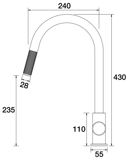
IDK Vetro Sink Pull-Out Mixer Gooseneck A48.024.2.24 - Brushed Gunmetal
