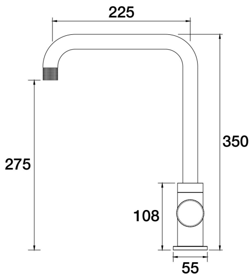
IDK Vetro Sink 90 Degree Mixer A48.025.1.26 - Black Sapphire
