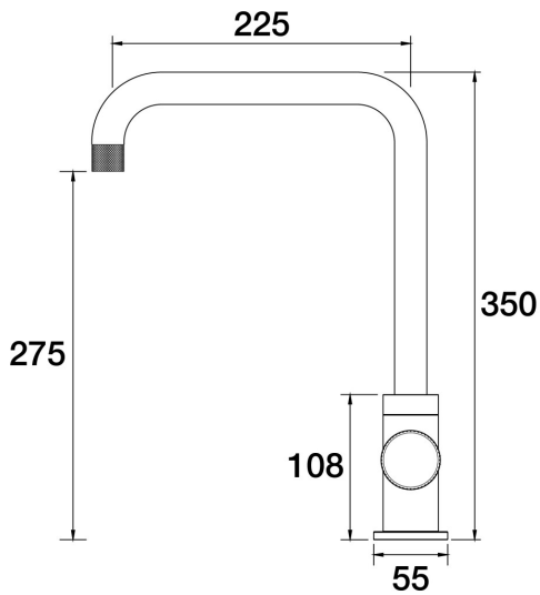
IDK Vetro Sink 90 Degree Mixer A48.025.1.45 - Native Brass
