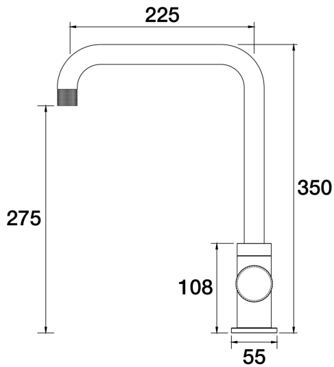
IDK Vetro Sink 90 Degree Mixer A48.025.1.52 - Burnished
