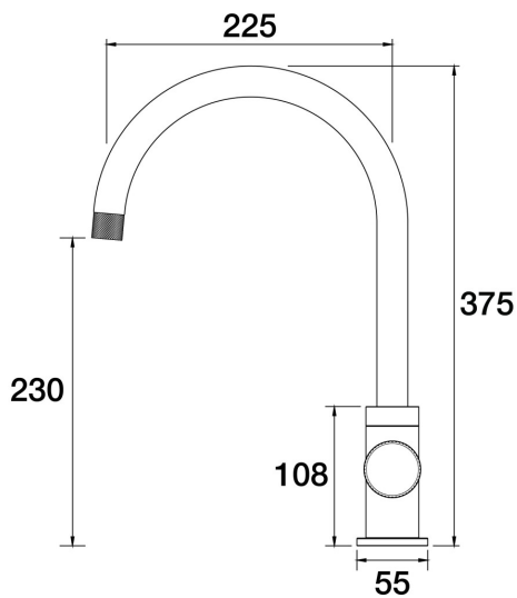
IDK Vetro Sink Gooseneck Mixer A48.026.1.26 - Black Sapphire
