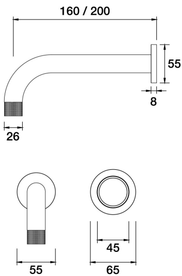
IDK Vetro Wall Mixer Basin Set 160mm outlet A48.033.2.67 - Vintage Brass
