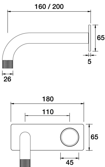
IDK Vetro Wall Bath Mixer Set 160mm outlet Incl. plate A48.041.1.27 - Satin Pearl
