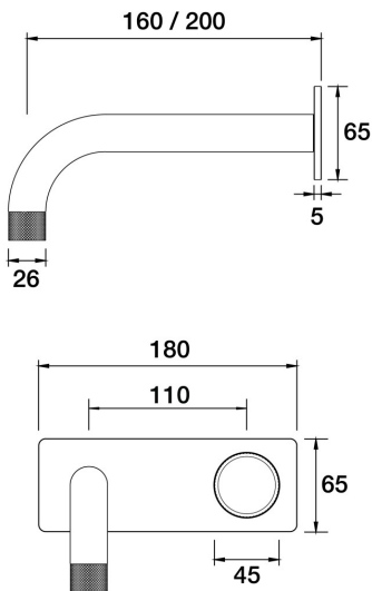
IDK Vetro Wall Bath Mixer Set 200mm outlet Incl. plate A48.041.2.19 - 23k Brushed Brass Gold
